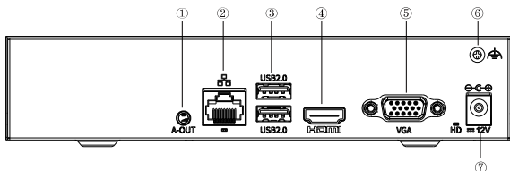
Figure 3-1 Non-PoE Device
