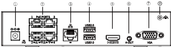
Figure 3-2 PoE Device
