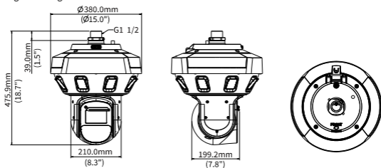
Figure 3-2 High-mounted MultiView Network PTZ Camera -- 8-inch model
