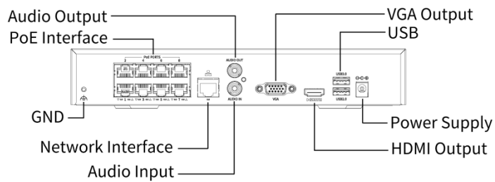
[NVR501-08B-P8]
