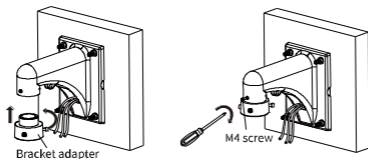
Bracket adapter
