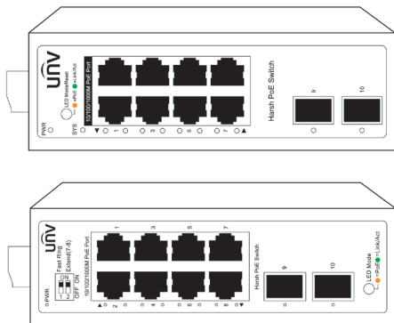
Figure 2-2 10 port 1000Mbps switch
