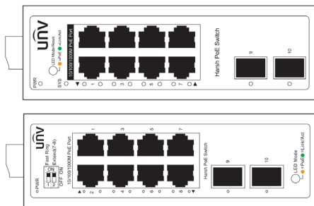
Figure 2-2 10 port 1000Mbps switch
