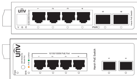
Figure 2-1 6 port 1000Mbps switch
