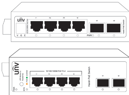
Figure 2-1 6 port 1000Mbps switch
