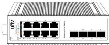
Figure 2-8 12 port 1000Mbps switch
