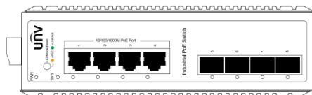
Figure 2-2 8 port 1000Mbps switch
