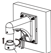
Bracket adapter
