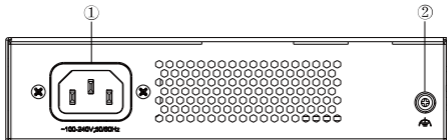
Rear Panel
